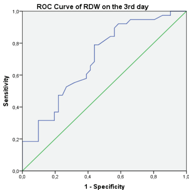
Figure 1. Receiving operator curve analysis of RDW3 value in predicting mortality
